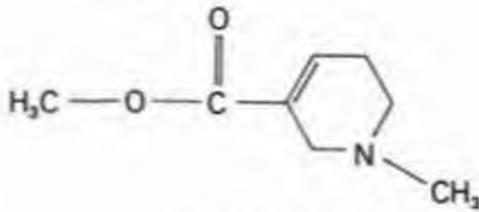
ARECOLINE
